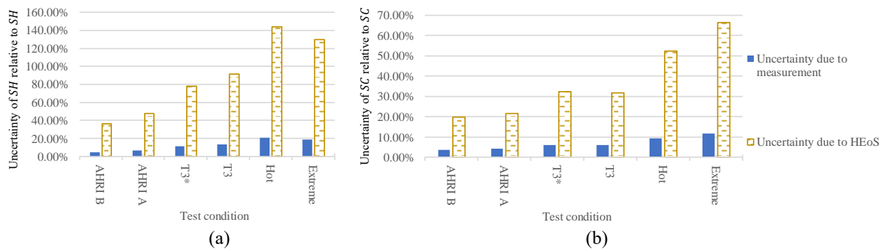
Figure 2: Comparison of (a) SH and (b) SC uncertainty due to measurement and HEoS
