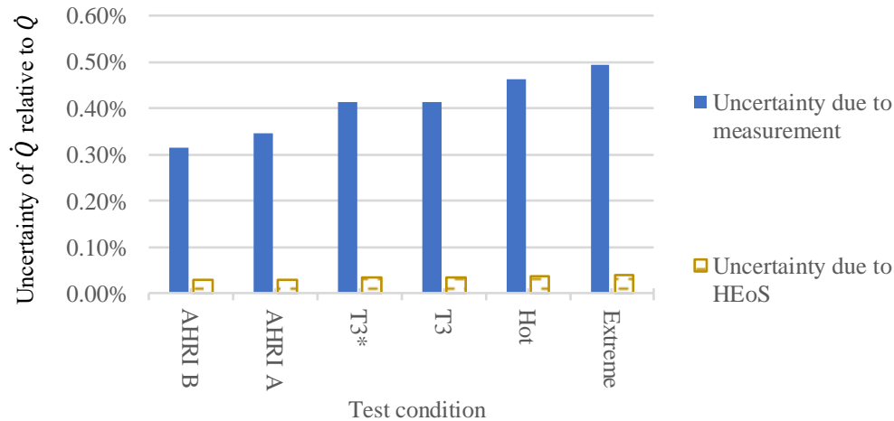
Figure 1: Comparison of heat transfer rate uncertainties due to measurement and due to HEoS
