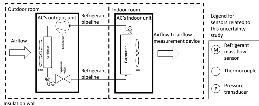
Figure 1: Test setup of a split air conditioner in environmental chambers
