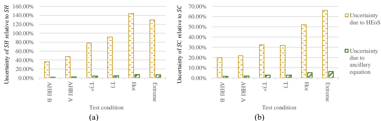
Figure 3: Comparison of (a) SH and (b) SC uncertainties due to HEoS and the ancillary equation
